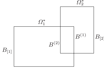
Fig. 1.3. Boundary segments for an overlapping decomposition
