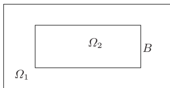
Fig. 6.2. Two subdomain non-overlapping decomposition
