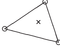
Fig. 11.10. Example of an interpolation stencil
